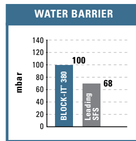
BLOCK-IT* 380 Fabric has higher hydrohead vs. the average of competitive SFS structures tested.
