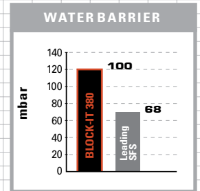
BLOCK-IT ® 380 Fabric has higher hydrohead vs. the average of competitive SFS structures tested.
