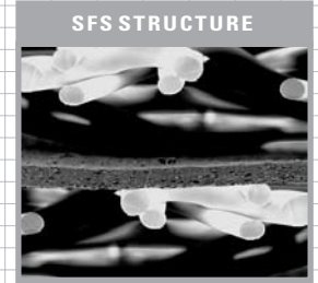
Cross-section of BLOCK-IT ® 380 spunbond/film/spunbond laminate.
