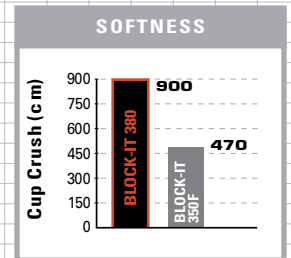
Due to the bicomponent fiber technology, BLOCK-IT ® 380 is nearly twice as soft as BLOCK-IT ® 350F.
